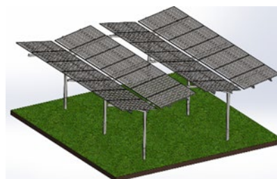
ARTEMIS beta
