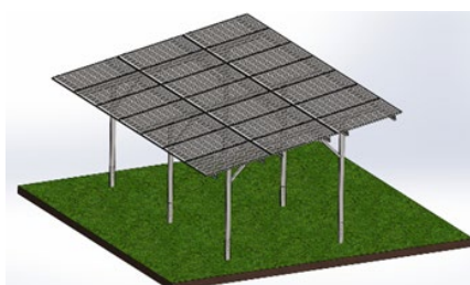
ARTEMIS alpha
